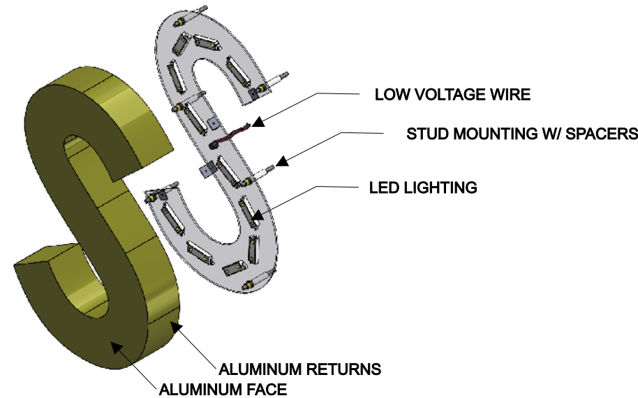
ISOMETRIC EXPLODED VIEW REVERSE LIT (HALO) CHANNEL LETTER
