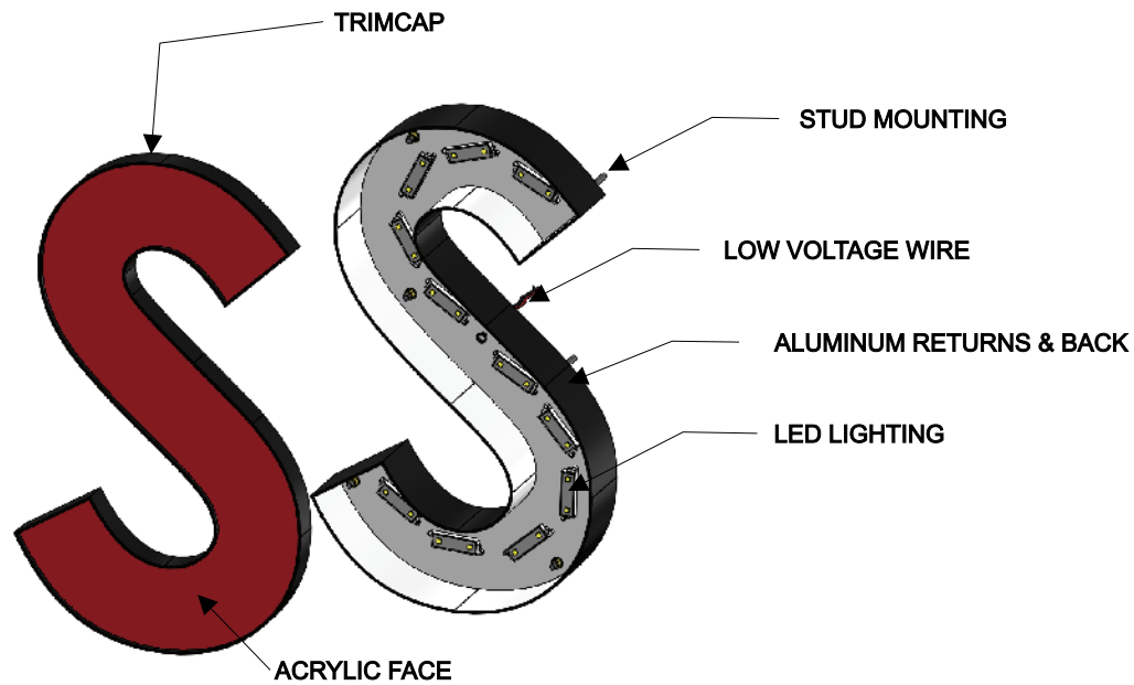
ISOMETRIC EXPLODED VIEW FRONT LIT CHANNEL LETTER
